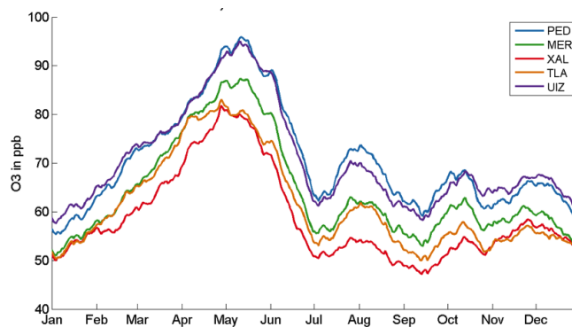
Figure 3. Annual cycles of surface ozone concentrations (ppb) for five observing stations for hours 12:00–16:00 LT (local time) from the RAMA network, 1986–2014. Observations are smoothed using a 30-day running mean.
