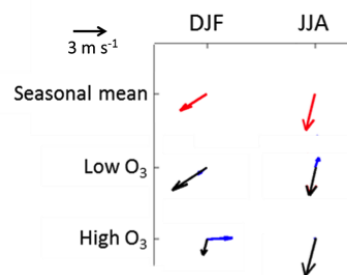
Figure 10. Mean 10 m winds at Tacubaya station (TCBY in Fig. 1) at 18:00 UTC (12:00 LT). Mean surface wind vectors for each season, DJF and JJA, are on row one and indicated by red arrows. Mean (black arrows) and anomaly (blue arrows) vectors for the MJO phases associated with lowest surface ozone (phase 8 in DJF and phase 1 in JJA) are on the middle row. Mean (black arrows) and anomaly (blue arrows) vectors for the MJO phases associated with highest surface ozone (phase 2 in DJF and phase 6 in JJA) are on the bottom row. Note that the mean winds for low ozone in DJF and high ozone in JJA are very similar to the seasonal mean winds, so the anomaly (blue) vector is very small. All wind data are from NOAA National Centers for Environmental Information, 1986–2014.
