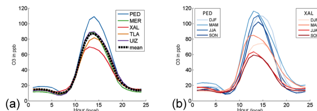
Figure 2. (a) Diurnal cycle of surface ozone concentrations (ppb) at five observing stations (colored lines), as well as the mean (black dotted line) for all seasons, 1986–2014. (b) Diurnal cycle of surface ozone concentrations for Pedregal (PED; blue lines) and Xalostoc (XAL; red lines) by season from the RAMA network, 1986–2014.
