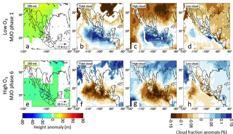
Figure 9. As in Fig. 8, but for summer days in active MJO phase 1 ( a–d ) and active MJO phase 6 ( e–h ). Phases 1 and 6 were the phases with lowest and highest respective summer ozone concentrations in Mexico City.
