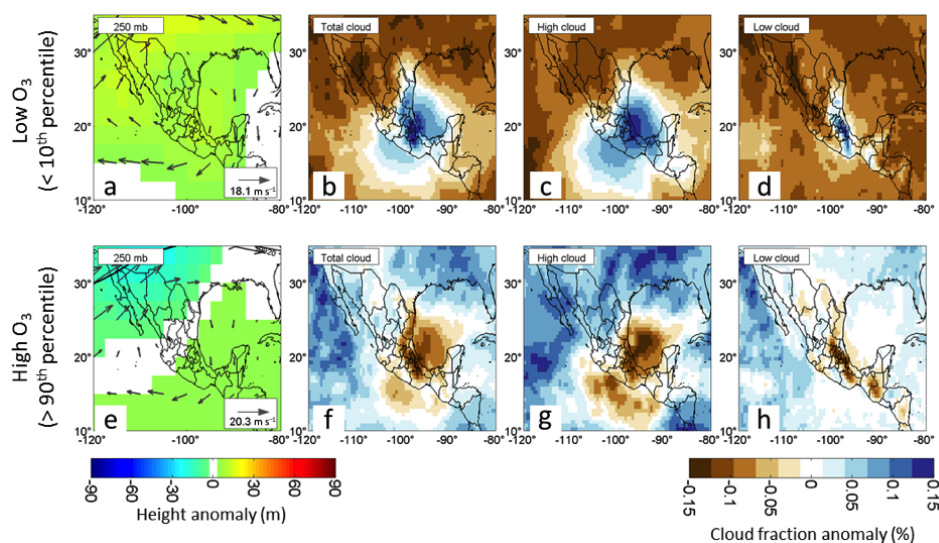
Figure 6. As in Fig. 5, but for summer (JJA) days.
