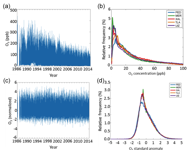
Figure 4. (a) Hourly observations of surface ozone concentrations (ppb) at Pedregal station (PED in Fig. 1). (b) Relative frequencies (in %) of hourly ozone concentrations (ppb) at five observing stations, 1986–2014. (c) Standard anomalies of hourly surface ozone concentrations at PED. (d) Relative frequencies (in %) of standard anomalies of hourly ozone concentrations at five observing stations from the RAMA network, 1986–2014.
