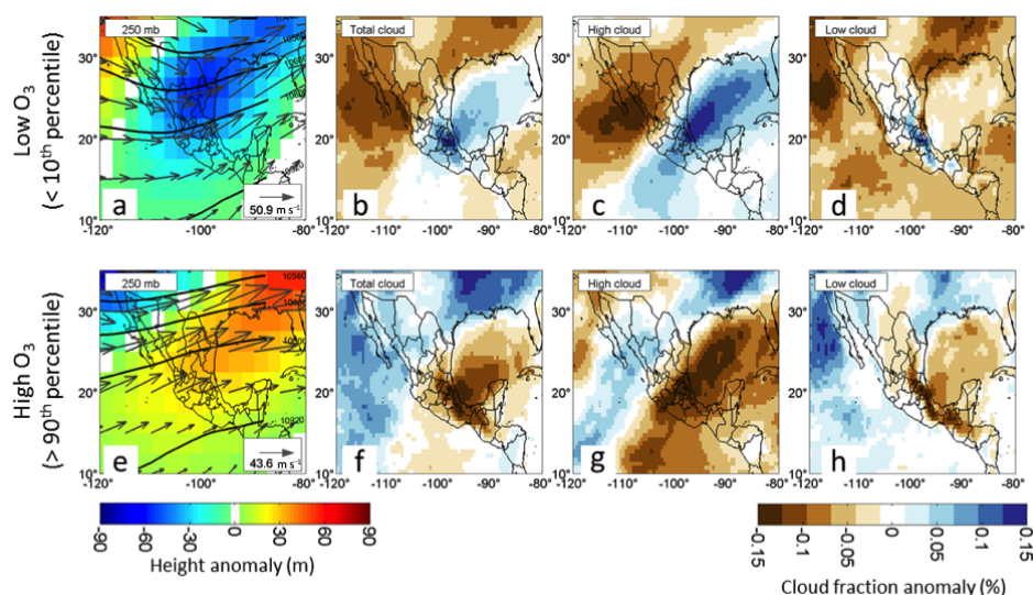
Figure 5. (a) Height (contoured, in m), height anomalies (shaded, in m), and mean winds (vectors) at 250 hPa for winter (DJF) days with standard anomalies of afternoon (12:00 to 16:00 LT) surface ozone at the five observing stations (Fig. 1) below the 10th percentile. (b–d) Anomalies (in %) of total cloud fraction, high cloud fraction, and low cloud fraction, respectively, for the same winter days with standard anomalies of afternoon surface ozone concentrations below the 10th percentile. (e–h) Same as in panels (a–d), but for winter days with mean afternoon surface ozone concentrations above the 90th percentile. Percentile calculations based on hourly observations from 1986–2014. Height, wind, and cloud fraction data from ERA-Interim; ozone concentrations from RAMA stations.
