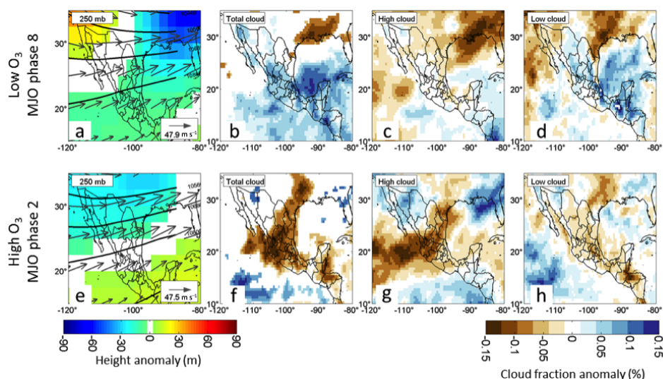
Figure 8. Composites of 250 hPa height (in m), height anomaly (in m), and mean wind ( a ), and total cloud fraction (in %; b ), high cloud fraction (in %; c ), and low cloud fraction (in %; d ) for winter days in active MJO phase 8. ( e–h ) Same as panels ( a–d ) but for winter days in active MJO phase 2. Phases 8 and 2 were the phases with lowest and highest respective winter ozone concentrations in Mexico City.
