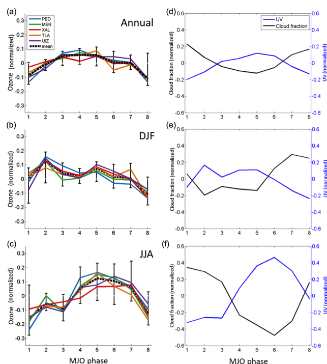
Figure 7. Mean standard anomalies of midday (hours 12:00–16:00 LT) surface ozone concentrations by active MJO phase for (a) annual, (b) DJF, and (c) JJA. Stations indicated by line color. Error bars indicate largest and smallest standard anomaly values for all stations; dashed black curve indicates mean value. All surface ozone observations from the RAMA network, 1986–2014. (d) Standard anomalies of UV radiation (blue curves) and total cloud fraction (black curves) for each active MJO phase for the entire year. (e, f) Same as panel (d) but for DJF and JJA, respectively. UV and cloud fraction data from ERA-Interim reanalysis, 1986–2014, for the grid closest to Mexico City.
