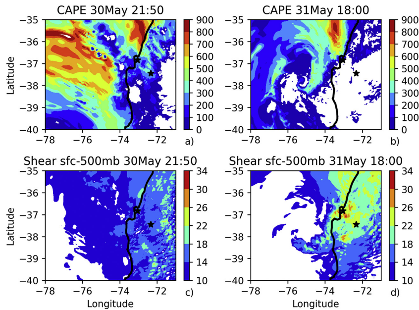
Fig. 14. (a)-(b) CAPE (in J\ kg^{-1} ) and (c)-(d) surface-to-500 hPa bulk wind difference (in m\ s^{-1} ), valid at 2150 UTC 30 May 2019 and 1800 UTC 31 May 2019, respectively. Both Los Angeles and Concepción are marked with a black star in each panel.
