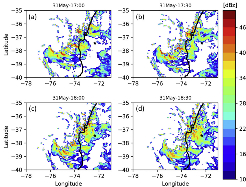
Fig. 12. Same as Fig. 10 but for (a) 1700 UTC, (b) 1730 UTC, (c) 1800 UTC, and (d) 1830 UTC 31 May 2019.
